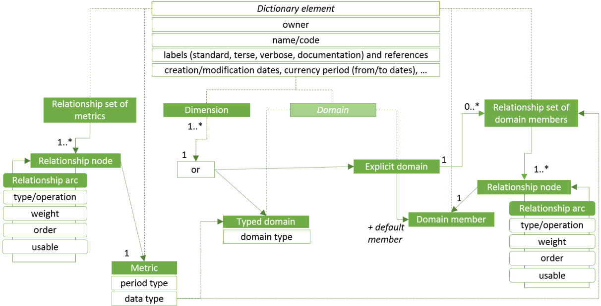
Figure 1. DPM dictionary
